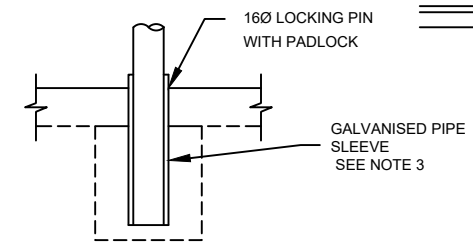
SLEEVE DETAIL (FOR REMOVABLE BOLLARD ONLY)
