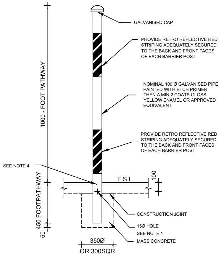
BOLLARD DETAIL
