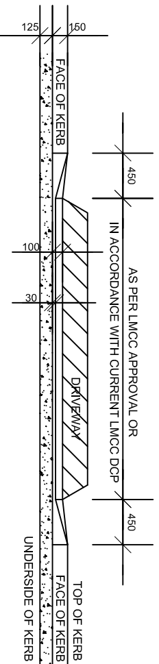
SECTION "A-A"
