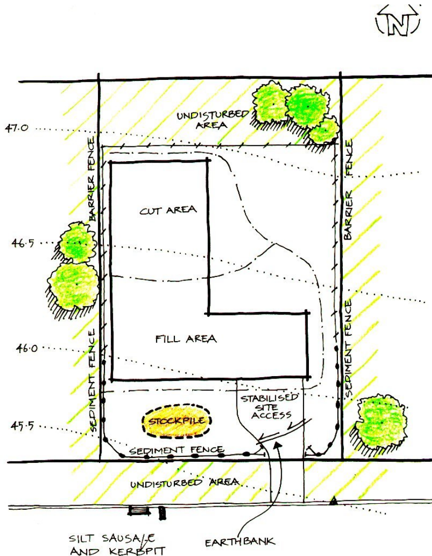
Figure 1 - Example of an Erosion and Sediment Control Plan on a sloping site and classed as development of 250m 2 to 1000m 2
