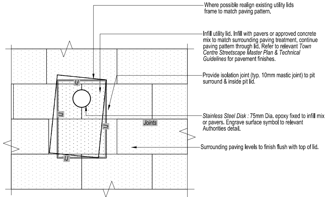
D1 Utility Lid in pavement (town centres) typical layout scale 1:20
