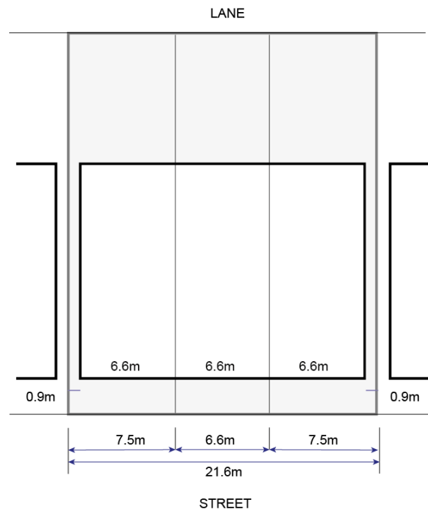
Figure 1 - Side setbacks for 'sets' of attached or abutting terraces
