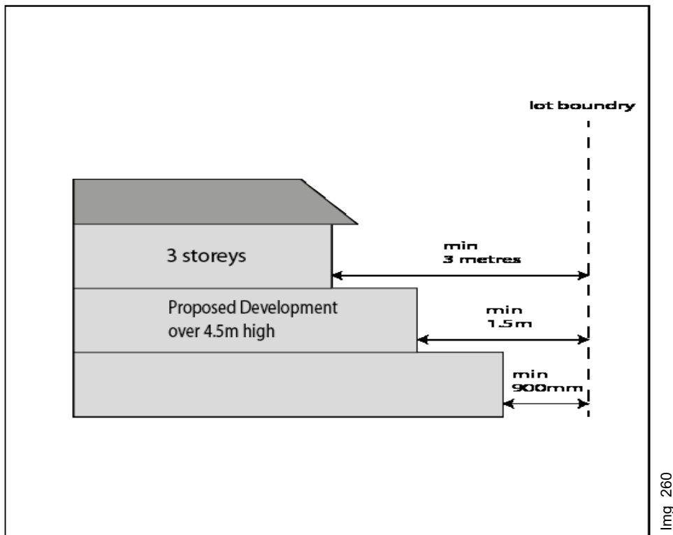
Figure 1 Side Setback for community title subdivision dwellings in E4 zone
